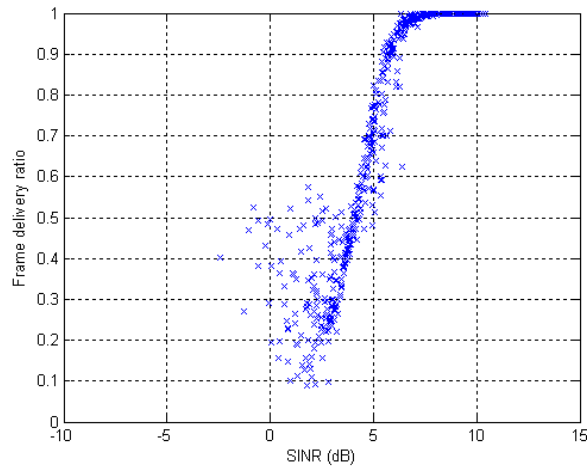
Fig. 23. Relationships between FDR and SINR when we enabled each interfering station according to a Poisson distribution
