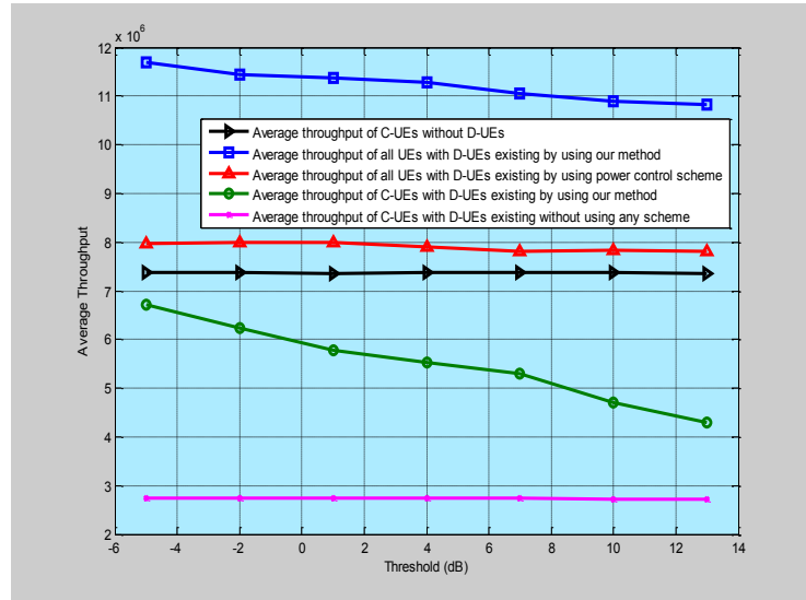
Fig. 13. (c) 50 cellular UEs vs. 50 D2D Ues
