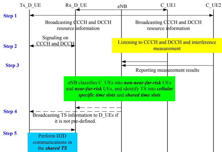
Fig. 10. Procedures of the proposed method to share cellular DL spectrum.
