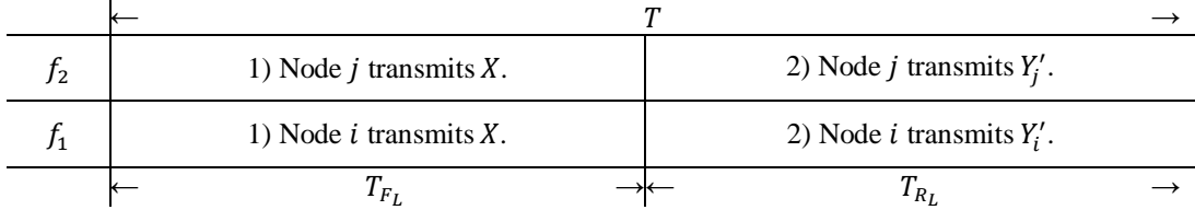
Fig. 2. Recourse Elements for Point-to-Point Link.
